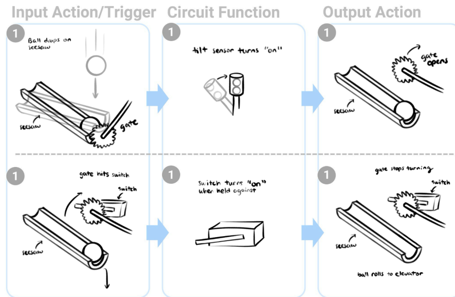
Figure 1. Electronics Circuit SportBot Action Summary Sketch
