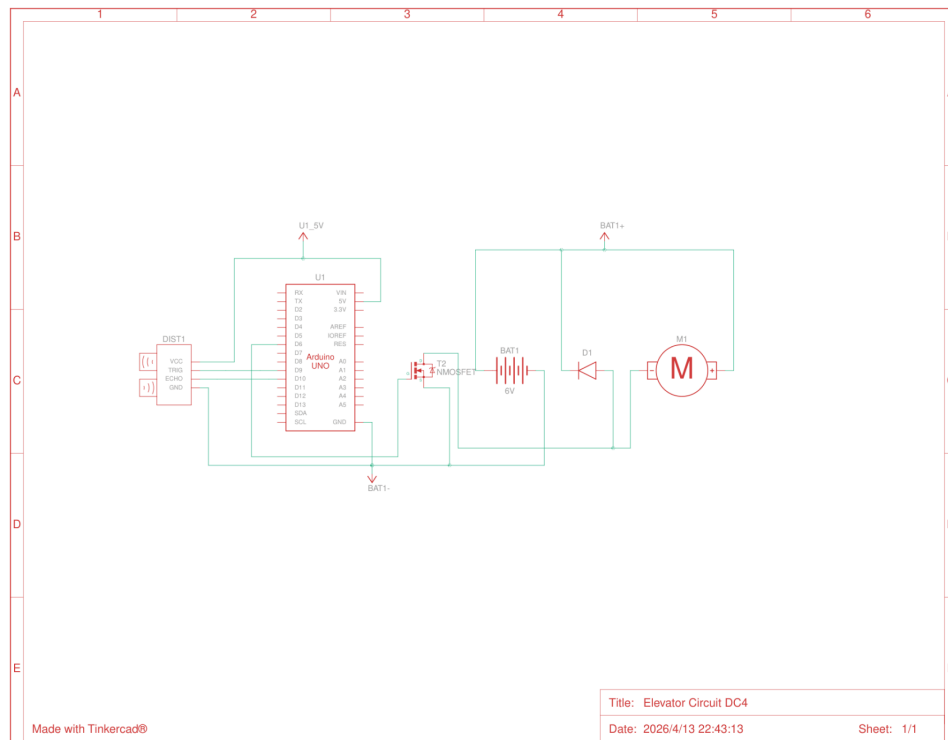
Figure 5. Microcontroller Circuit Schematic
